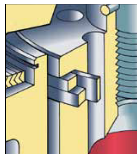
Triple Seal Ring
