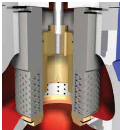
Typical Cascade flow path
