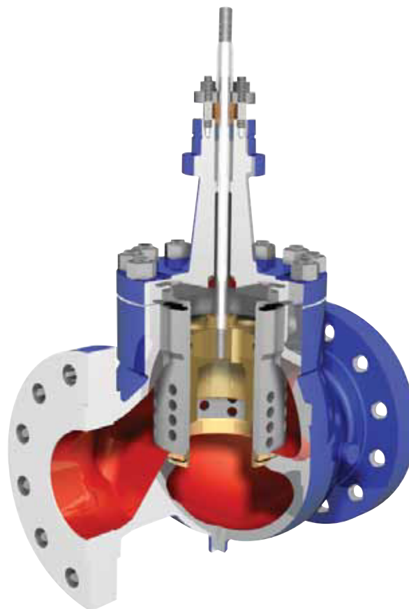
BV500/BV990 Cage Trim Valve with Multi-Flow cage
