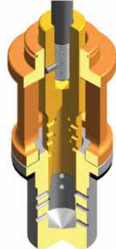
2-stage trim with diffuser
