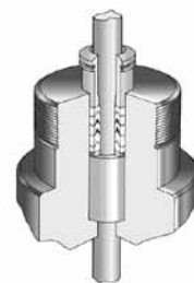
PTFE Chevron
